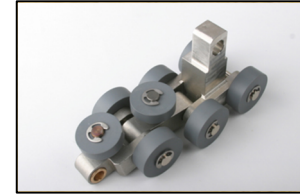
SLBN-5161 Chain Roller Assembly, Long Boss, 2.125" Center Height
