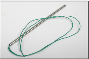
907747 Cart.Heater 220Vx1300W
